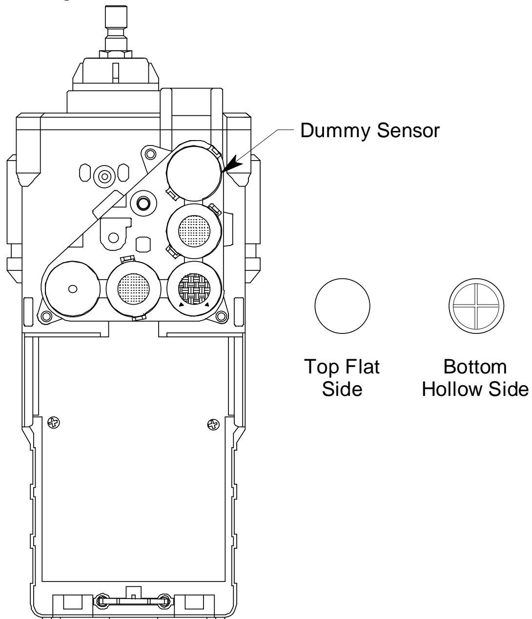
Figure 3: Dummy Sensors
