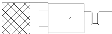
Figure 13: Dilution Fitting
