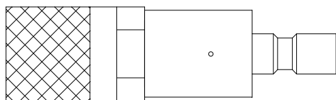
Figure 16: Dilution Fitting
